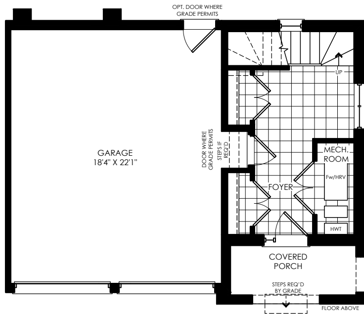
GROUND FLOOR ELEV. 'A'
