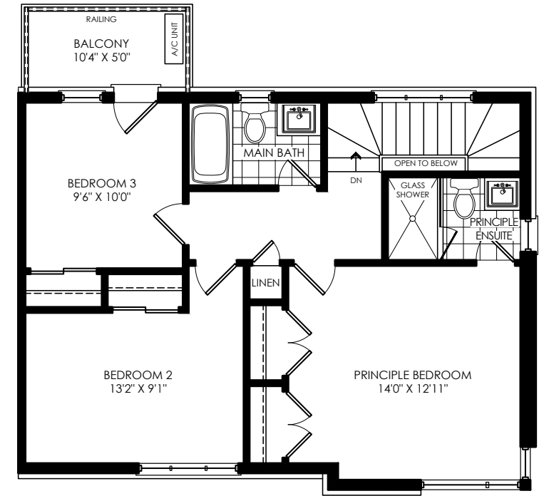
UPPER FLOOR ELEV. 'A'
