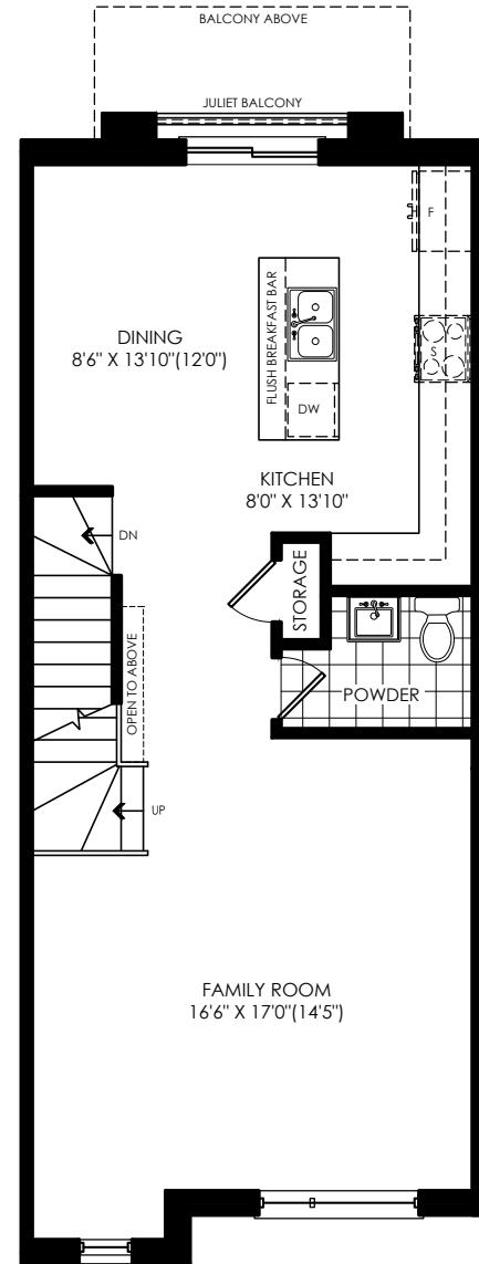
MAIN FLOOR ELEV. 'A'
