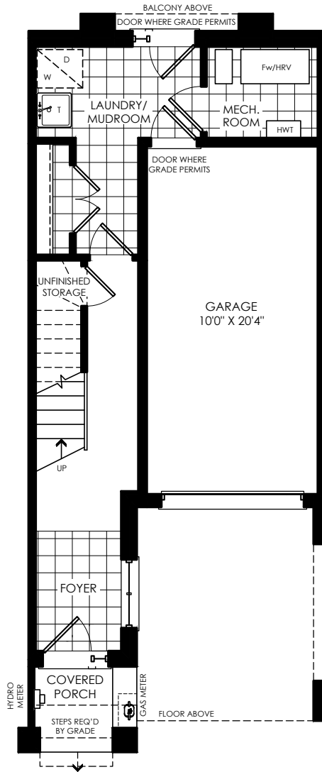
GROUND FLOOR ELEV. 'A'
