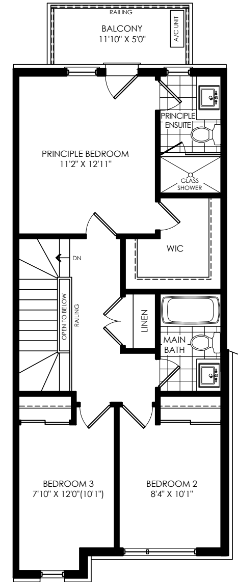
UPPER FLOOR ELEV. 'A'
