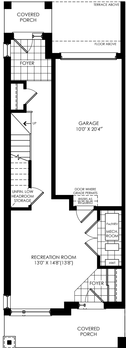
GROUND FLOOR ELEV. 'A'
