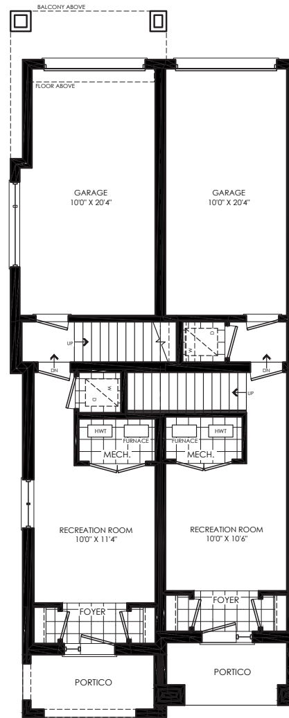
MODIFIED TH-1 ELEV 1 GROUND FLOOR PLAN
