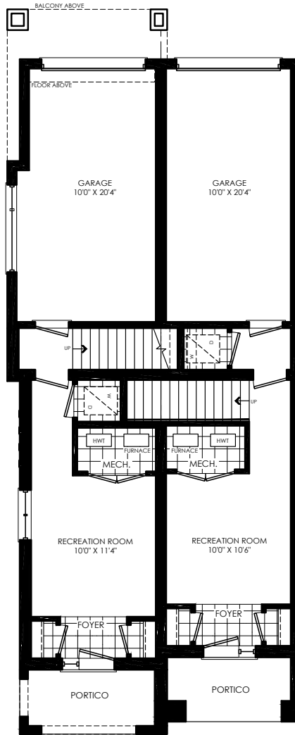
TH-1 ELEV 1 GROUND FLOOR PLAN
