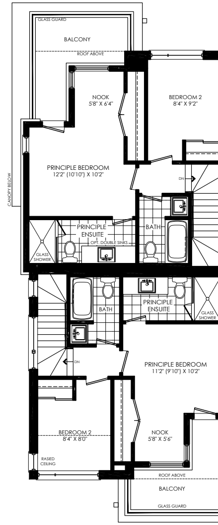
TH-2 UPPER FLOOR PLAN
