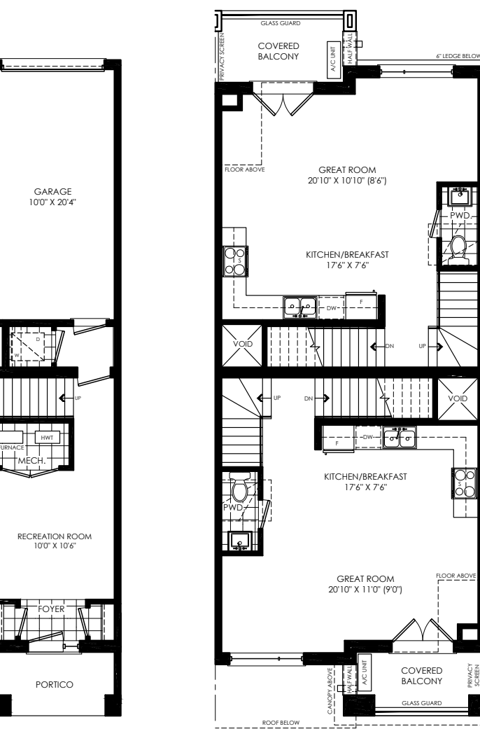
TH-2 ELEV 1 GROUND FLOOR PLAN
