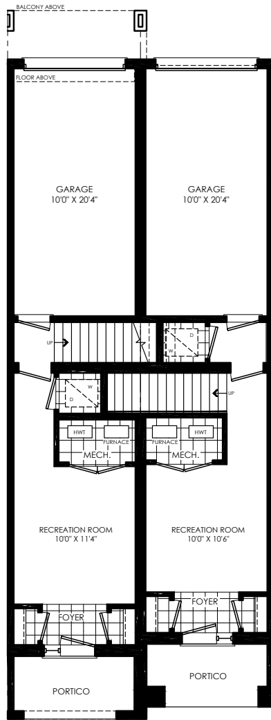
TH-1 ELEV 1 GROUND FLOOR PLAN
