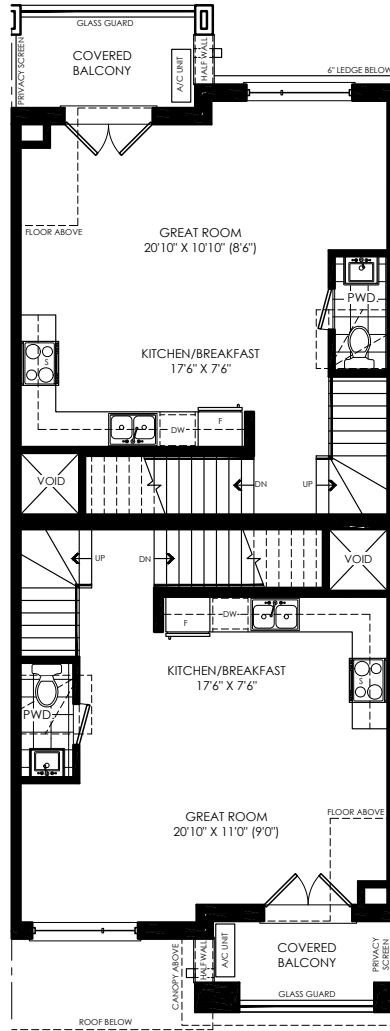
TH-2 MAIN FLOOR PLAN
