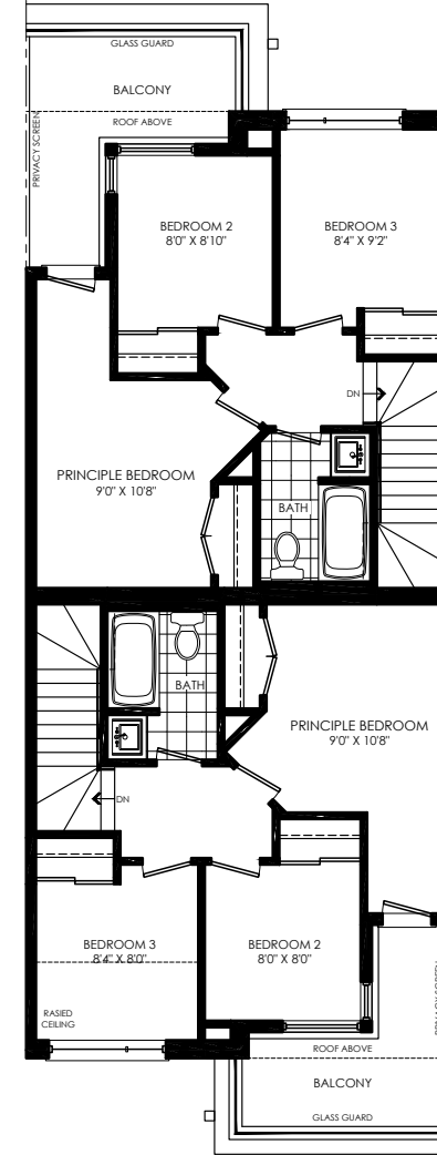
TH-2 (ALTERNATE 3 BEDROOM) UPPER FLOOR PLAN
